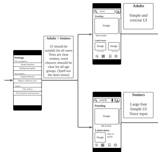
Figure 2: Modelling human-centric characteristics of end users (from (Jim et al., 2021)).
